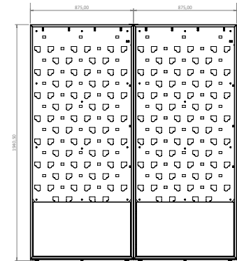
Double unit (1940mm x 1750mm x 600mm) Weight - 114 Kg (including foot plates)
