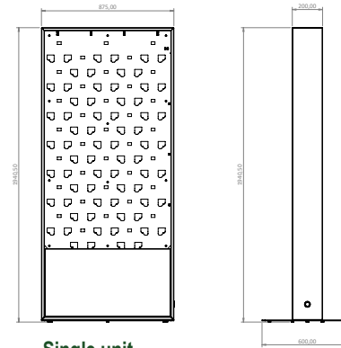
Single unit (1940mm x 875mm x 600mm) Weight - 57 Kg (incl foot plate)
