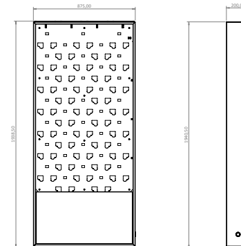
Wall unit (1940mm x 875mm x 200mm) Weight - 57 kg (incl wall bracket)
