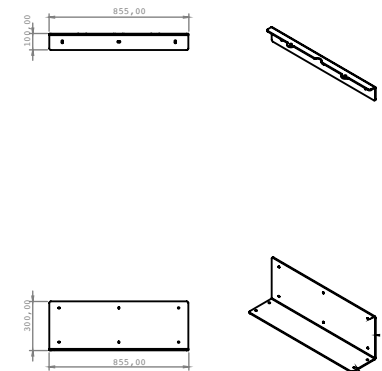
Wall brackets (855mm x 100mm) (855mm x 300mm) Weight - 26 Kg
